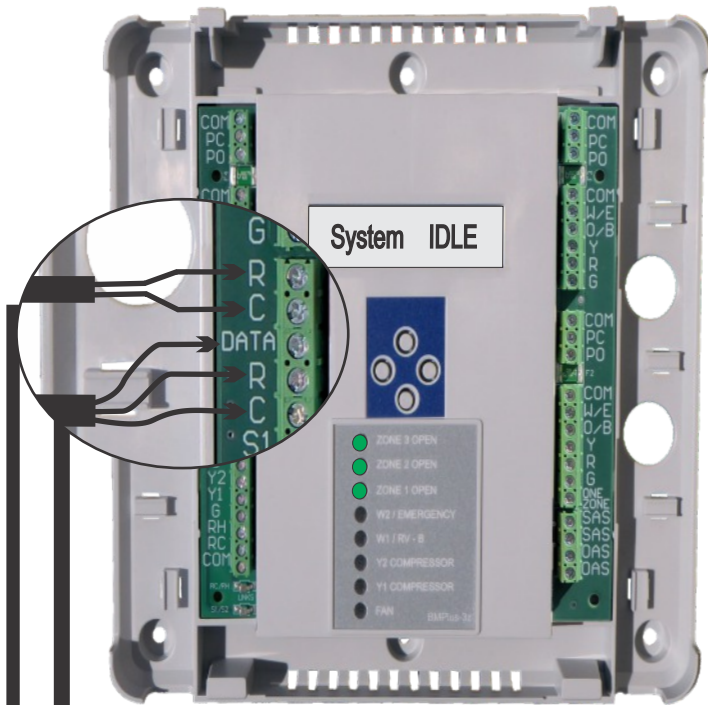
BMPlus-3z with 3 WiFi Tstats = 16va power load
