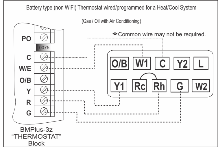
Figure 7 The diagram above reflects a "Battery" or "Power Robbing" thermostat, which means the thermostat only needs four wires. If you have five wires and the thermostat has a C terminal, make use of it and connect the 24v common wire anyway. See Notes below!
